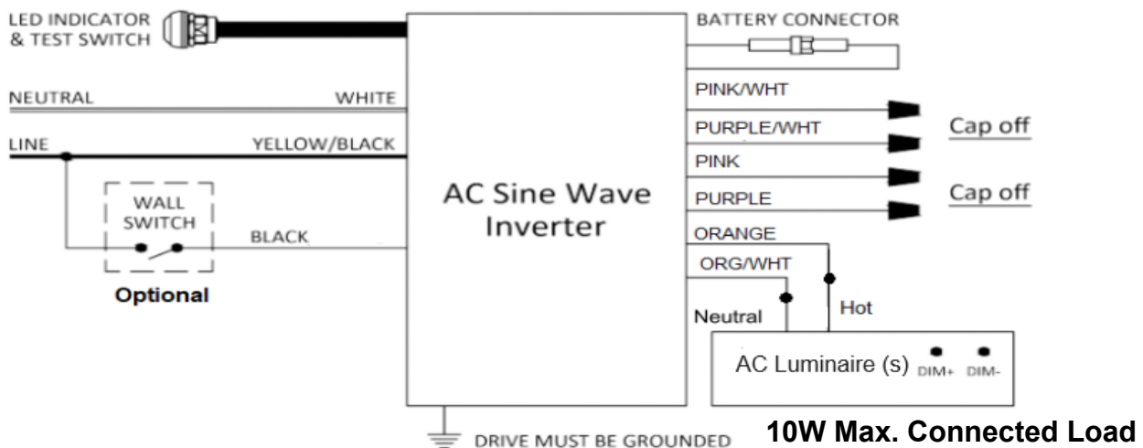
Figure B. Wiring Diagram without 0-10V Dimmer
